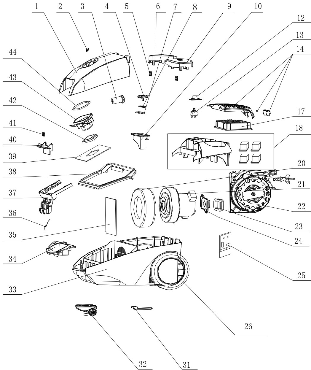
Exploded View for VC-H3609E
