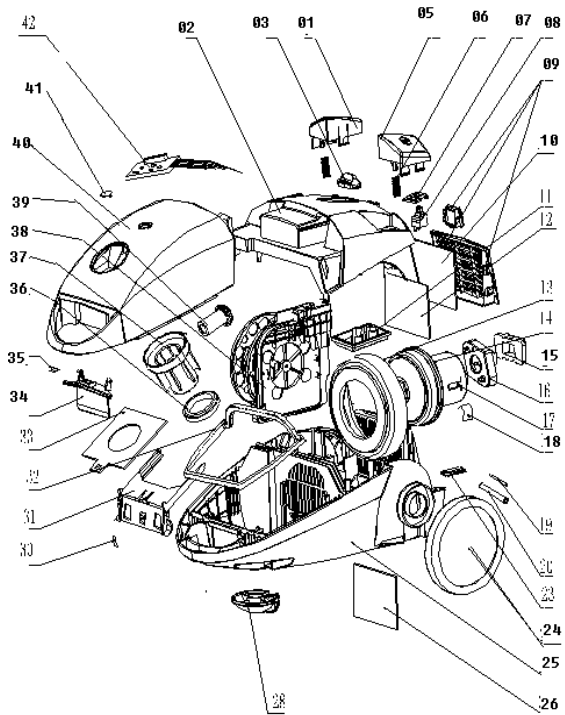
Exploded View for VC-H4203E AEG SMART460
