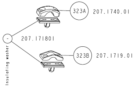
Different Types of Cable Clips/Clamps
