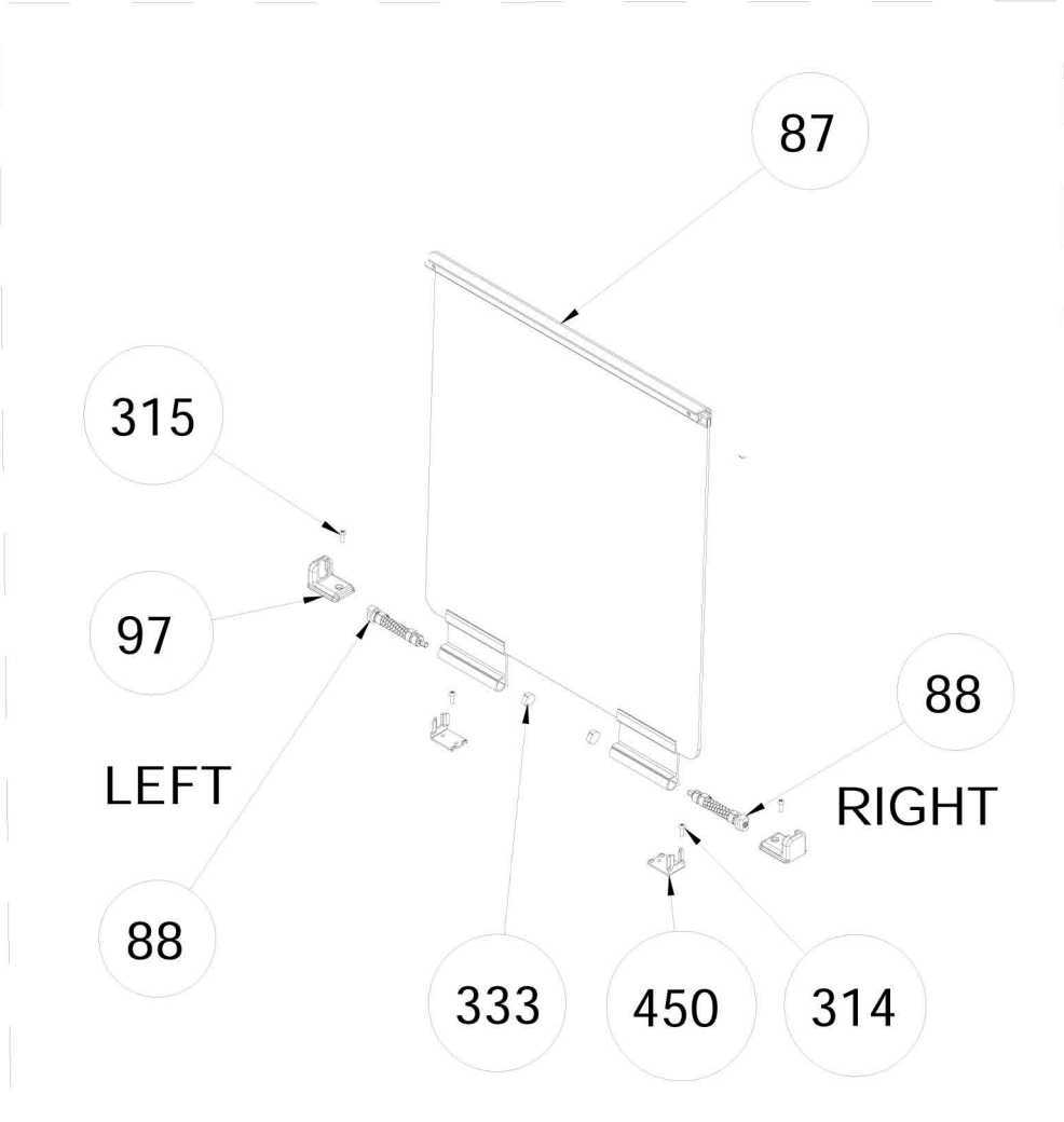
GLASS LID WITH SHORT PROFILE (OPTIONAL)
