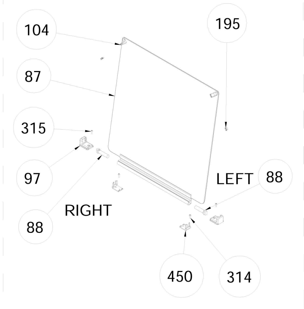
GLASS LID WITH BUMPER (OPTIONAL)
