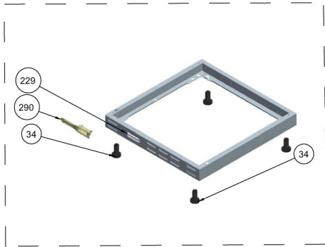
EXTRA BOTTOM SUPPORT ( WITH LOUVRES&BATTERY ) (OPTIONAL)
