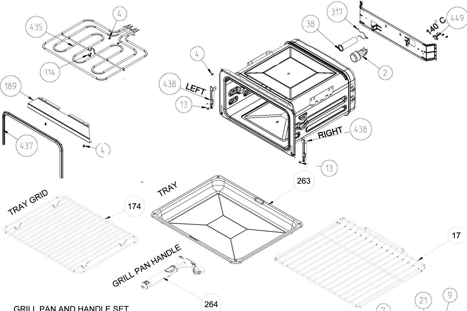
GRILL PAN AND HANDLE SET (TRAY SET FOR GRILL) POSITION NUMBER : 265 (OPTIONAL)
