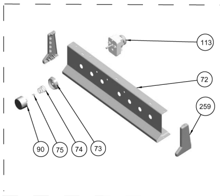
MECHANIC TIMER (OPTIONAL)
