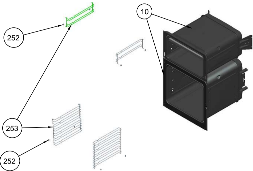
CAVITY ASSEMBLY WITH WIRE SHELF (OPTIONAL)
