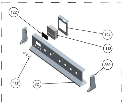
DIGITAL TIMER (OPTIONAL)
