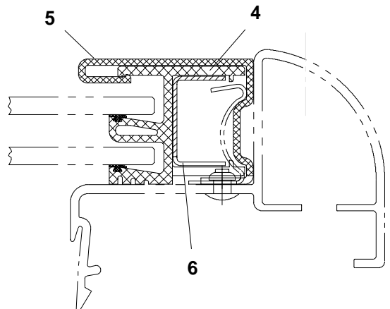
Detail Z
