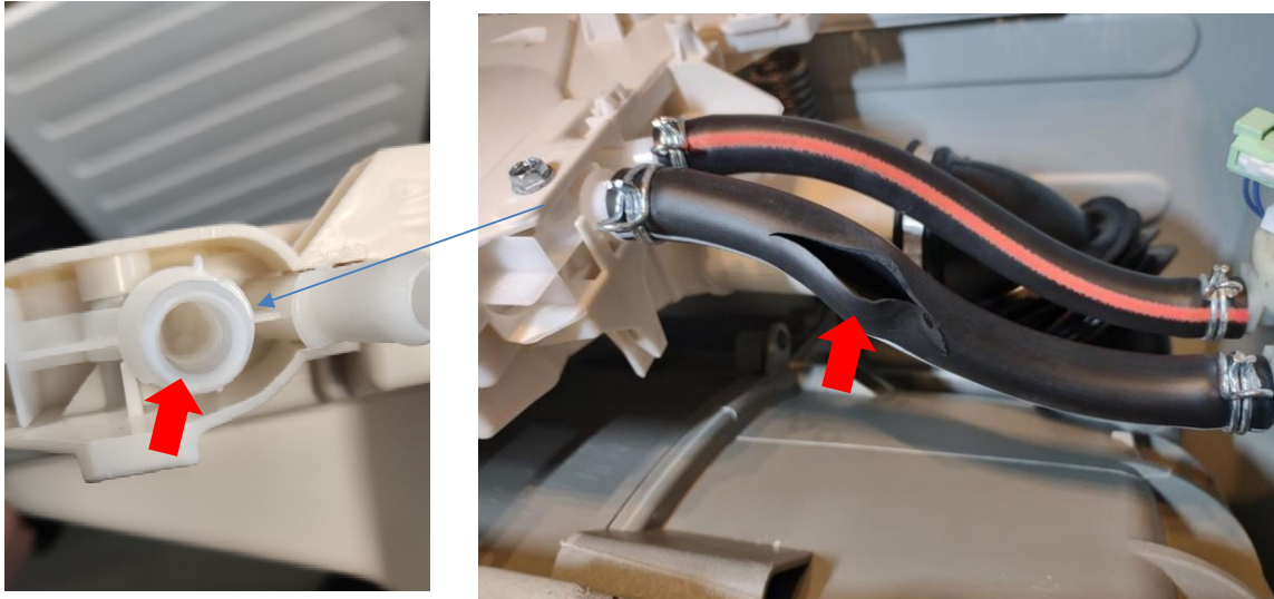
Clogged water distributor channel and cracked inlet valve pipe.
