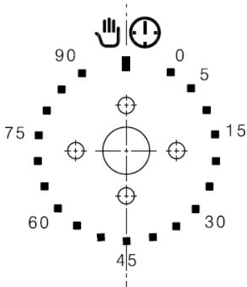
Minute minder and holes positions of old control panel
