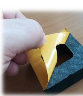
7. Fit the new sealing sponge and refit the silicon tube
