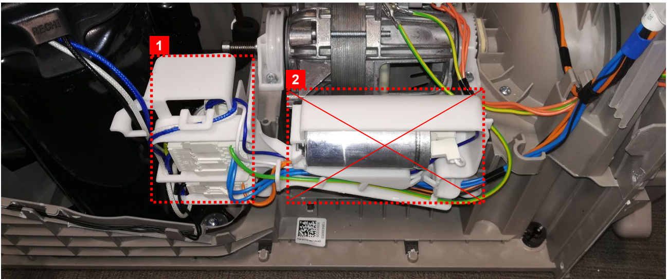
1 Replace capacitor from 10 \mu F to 20 \mu F
