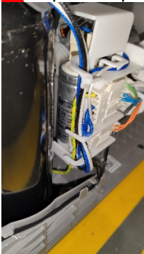
1 Replace capacitor from 10 \mu F to 20 \mu F
