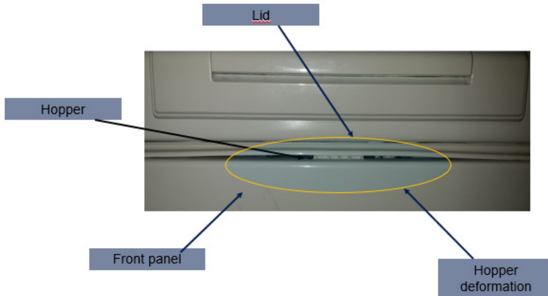
Photo1. Hopper deformation.
