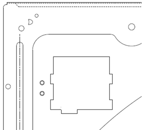
2. New back panel terminal hole.
