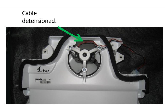
Cable detensioned. Correct position of the cable as shown in the picture. Cable should not be strained.
