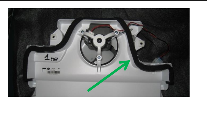
Align gasket to the shape of air channel.
