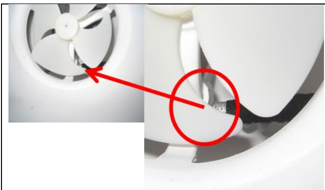
Evaporator battery tube should not be in contact with fan support.
