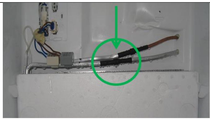
Pull down the evaporator battery tube to avoid contact with fan motor support.
