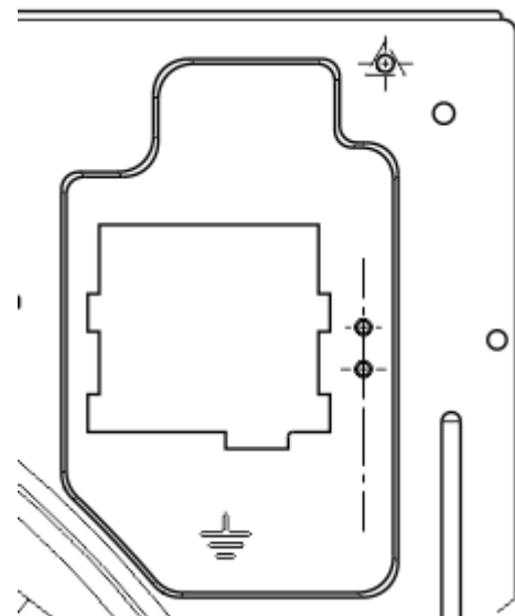
2. New back panel terminal hole.
