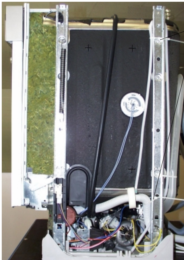
Cable fasteners
