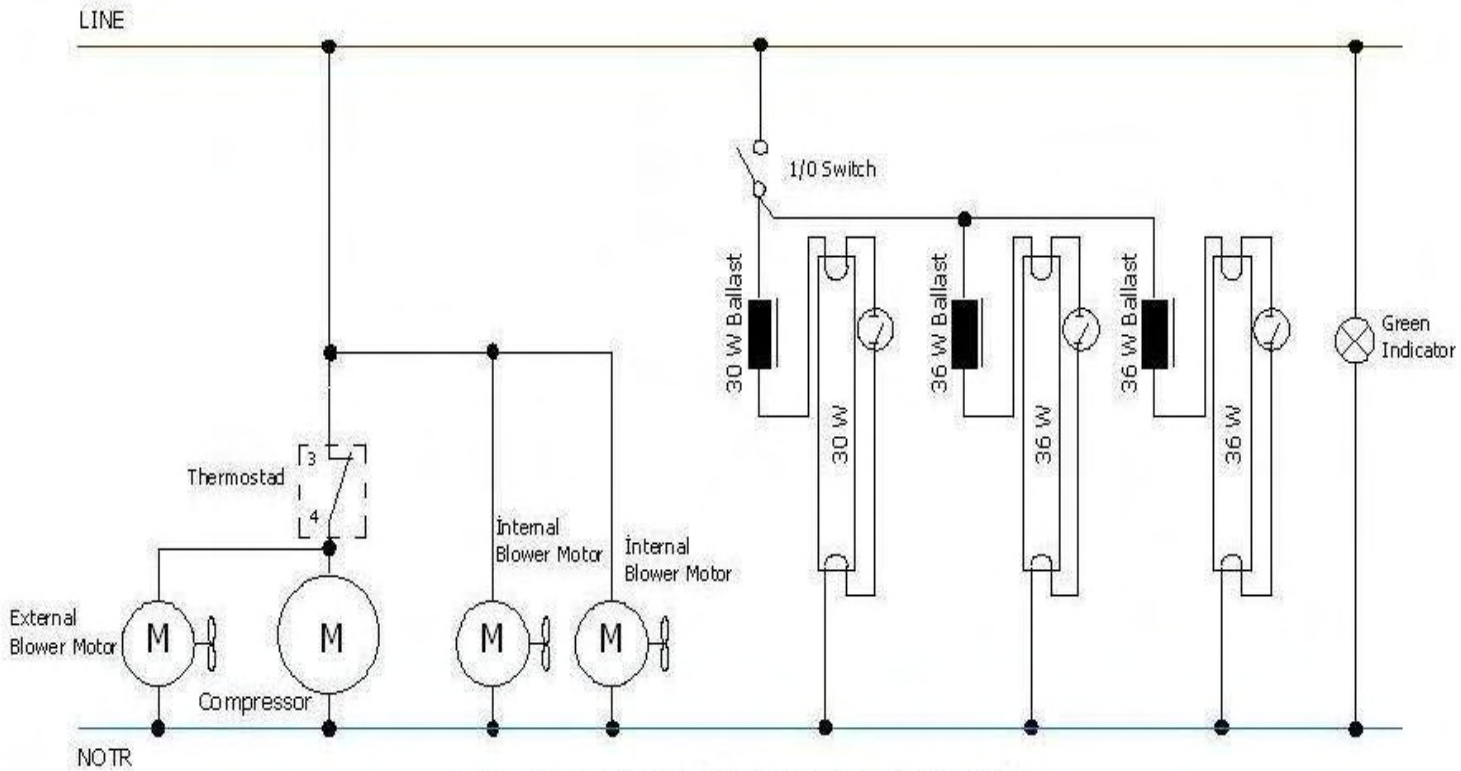
GD 880 CARRIER WIRING DIAGRAM
