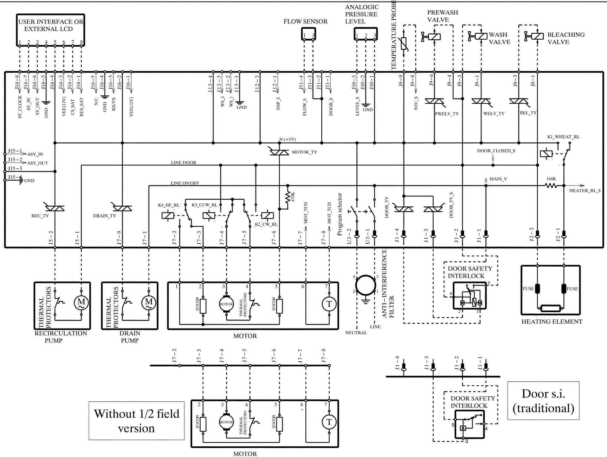
ELECTRIC DIAGRAM – EWM 2100
