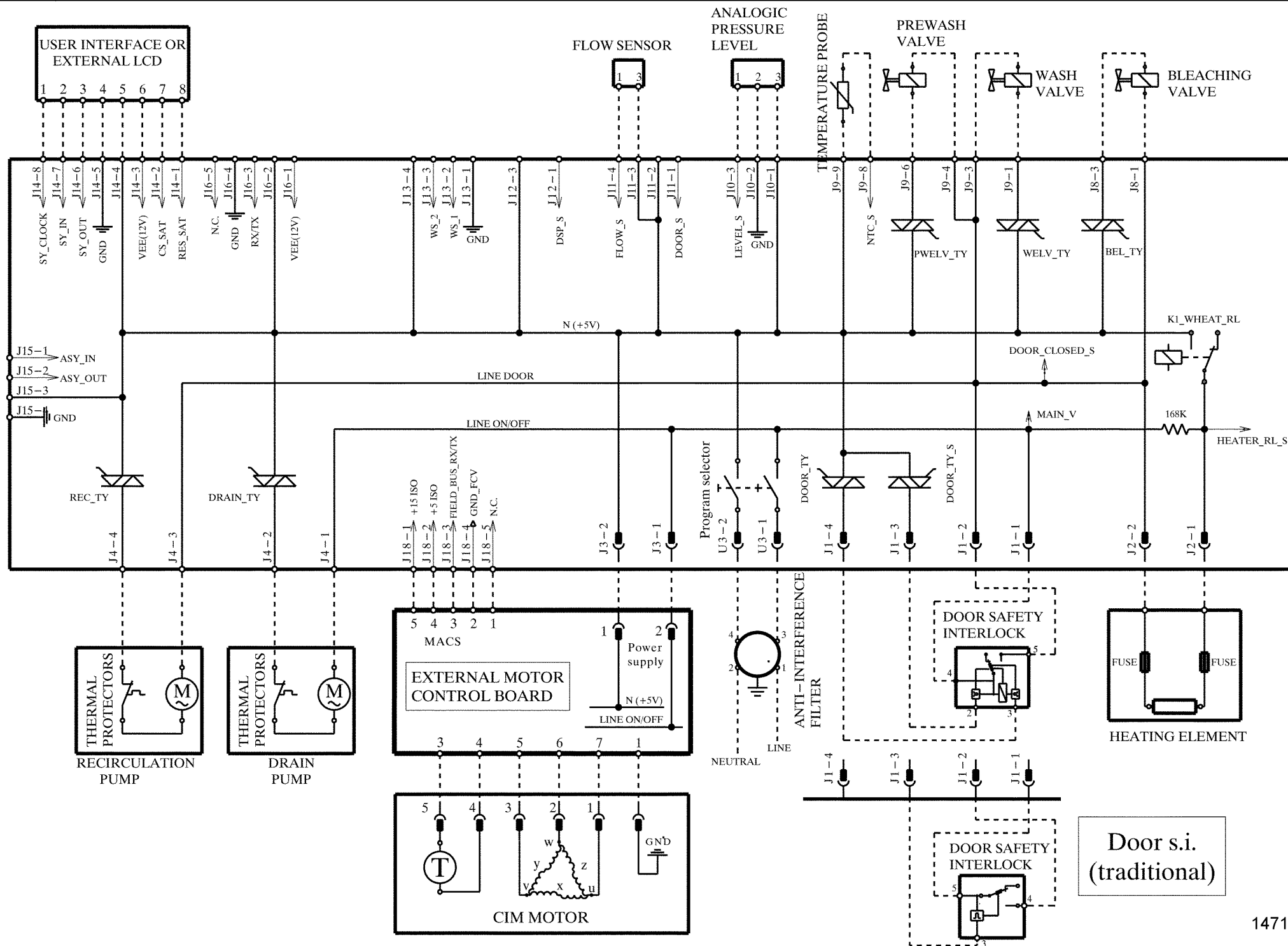
ELECTRIC DIAGRAM - EWM2500
