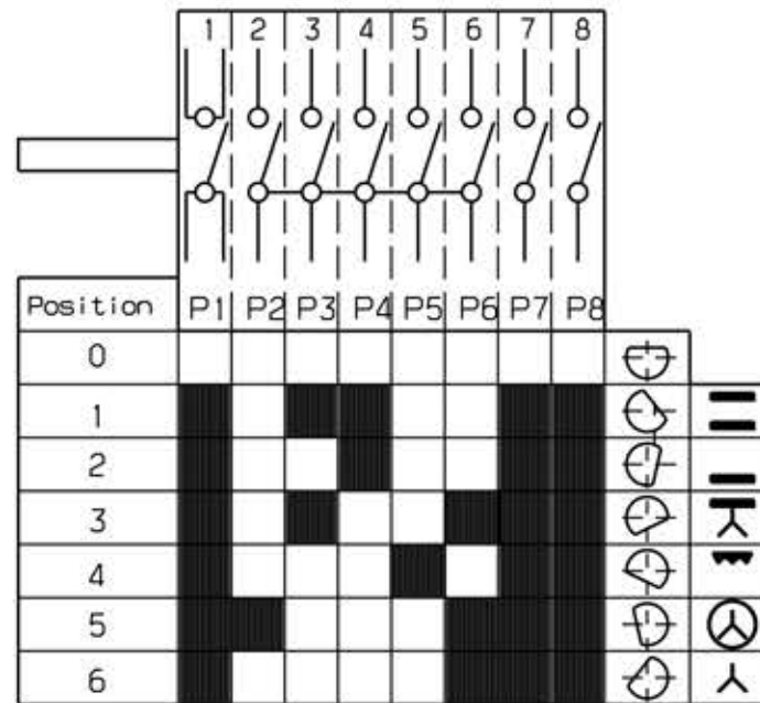
Switching diagram
