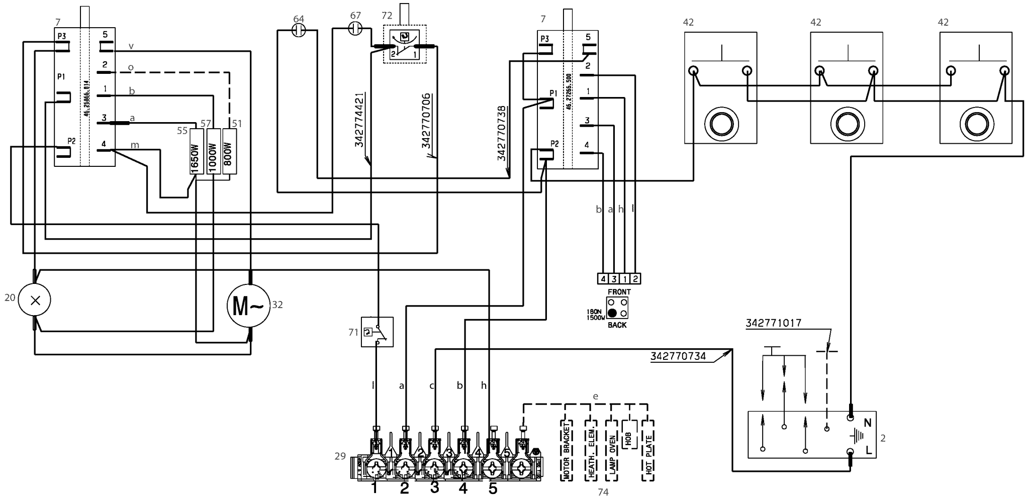
OVEN SWITCH
