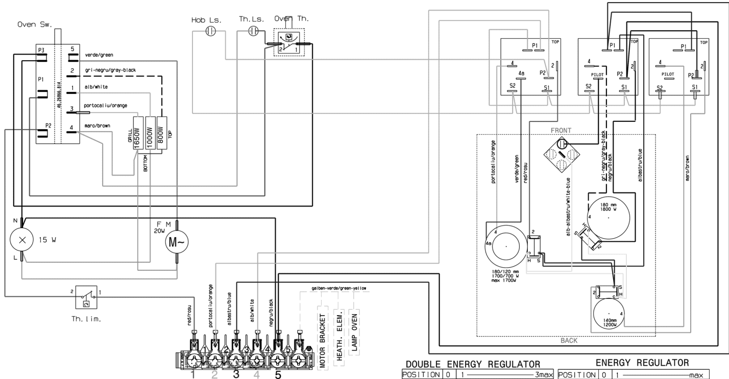
OVEN SWITCH
