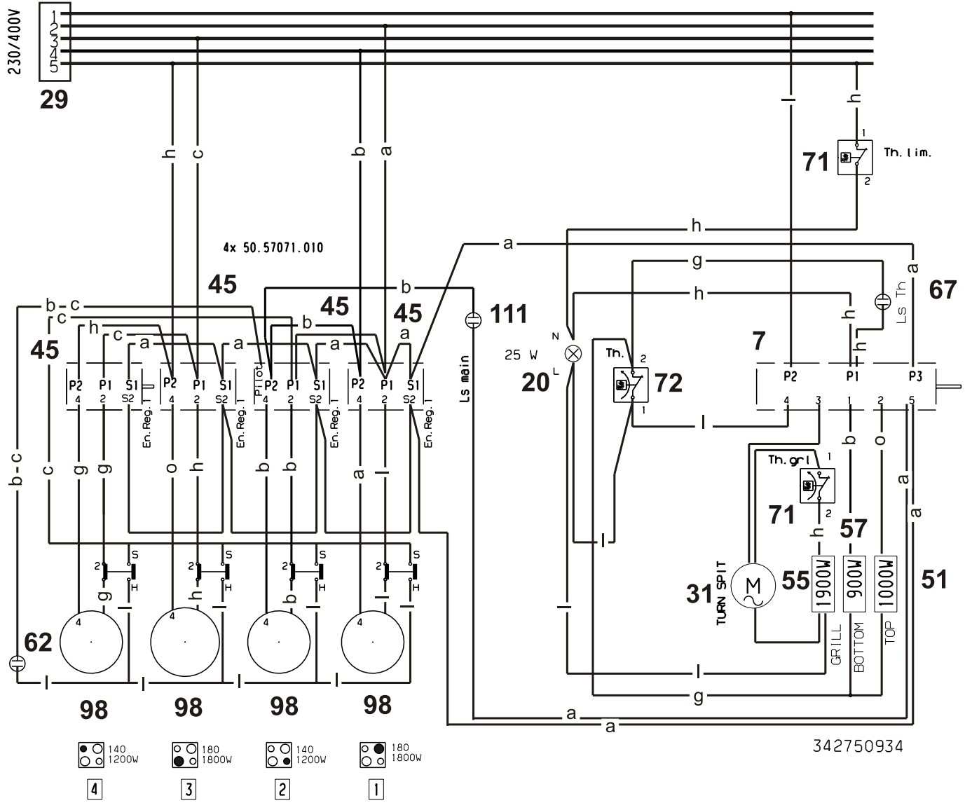
OVEN SWITCH 46.23866.862
