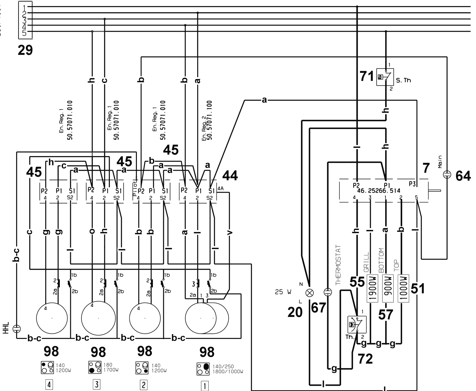
ENERGY REGULATOR
