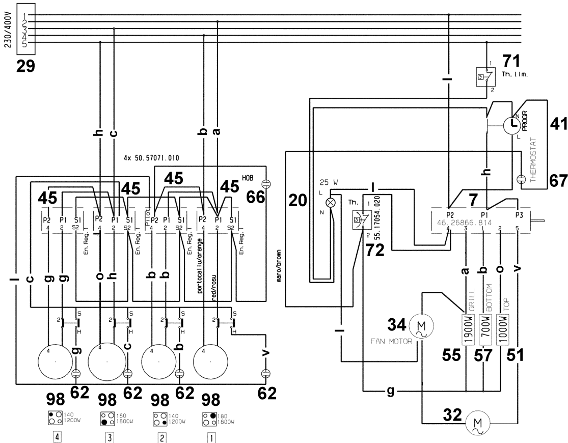
ENERGY REGULATOR
