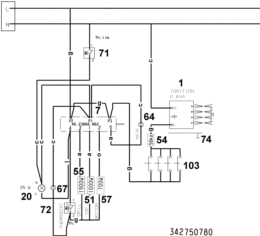
OVEN SWITCH 46.23866.862
