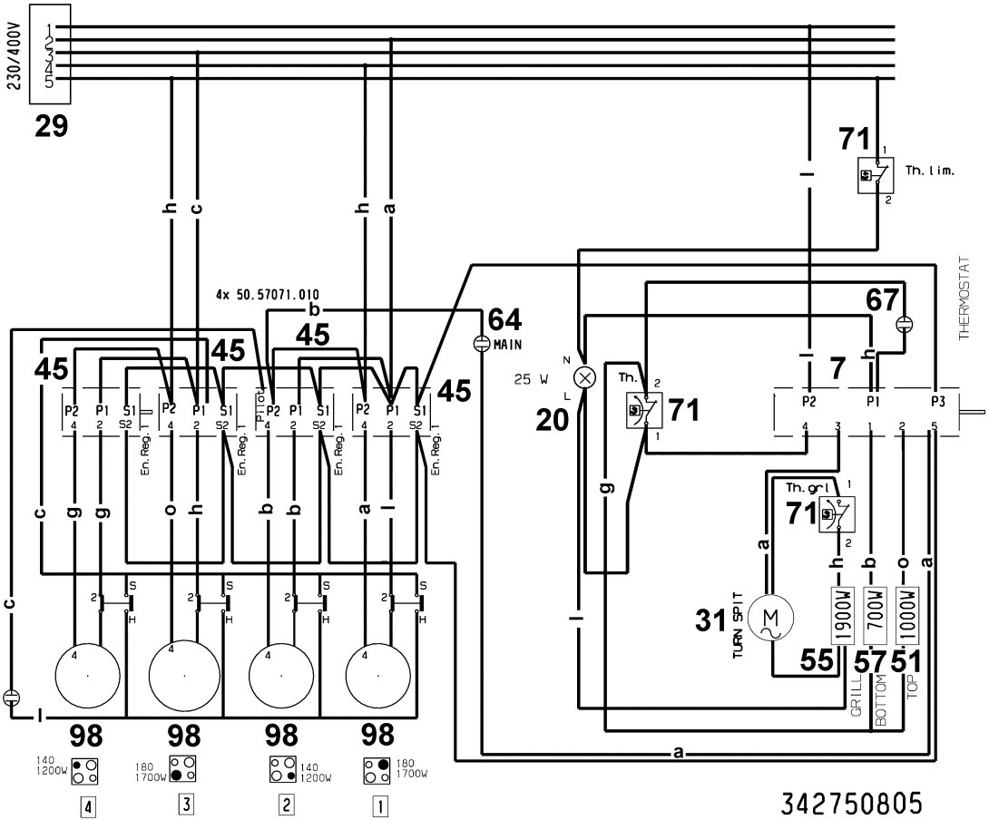
OVEN SWITCH 46.23866.862
