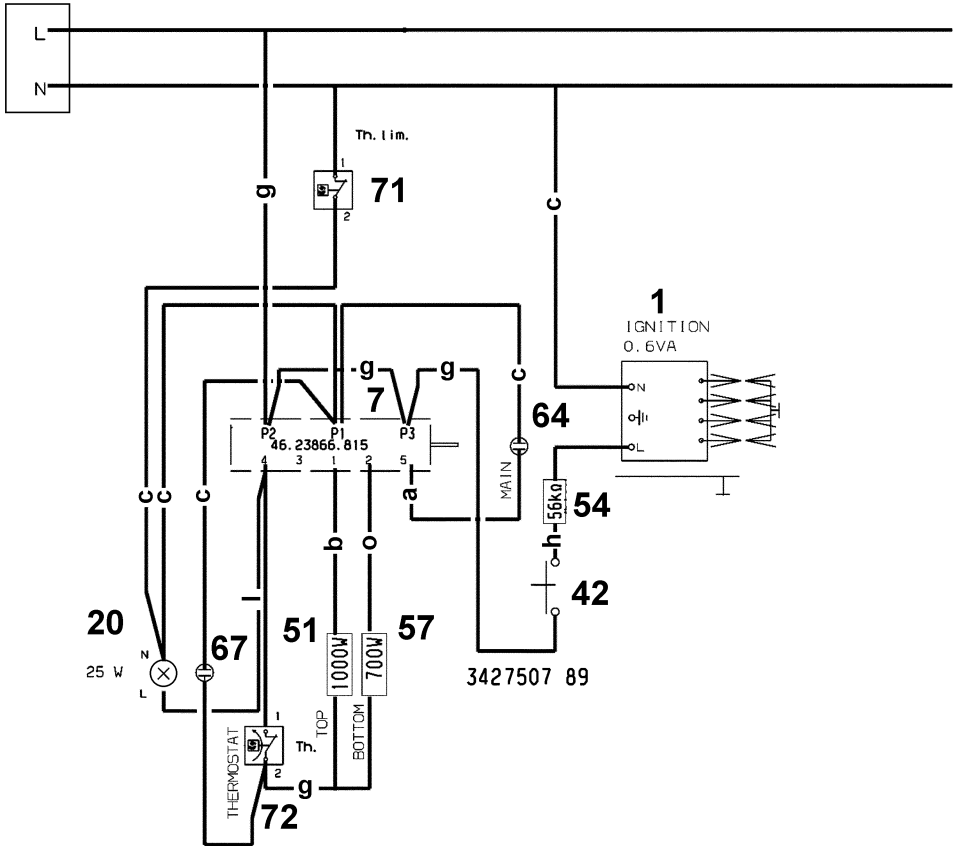
OVEN SWITCH 46.23866.815
