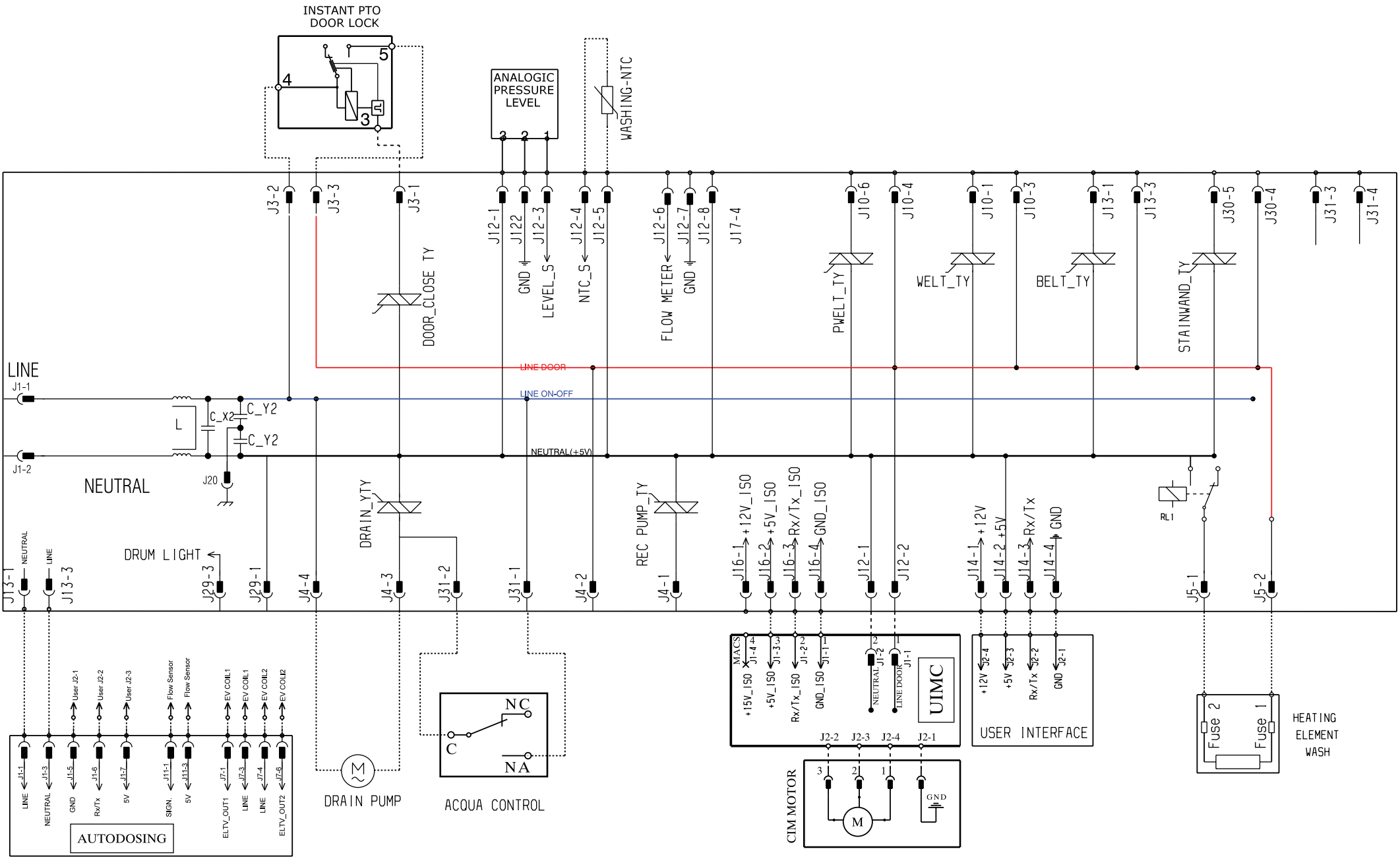
ELECTRIC DIAGRAM EVX14
