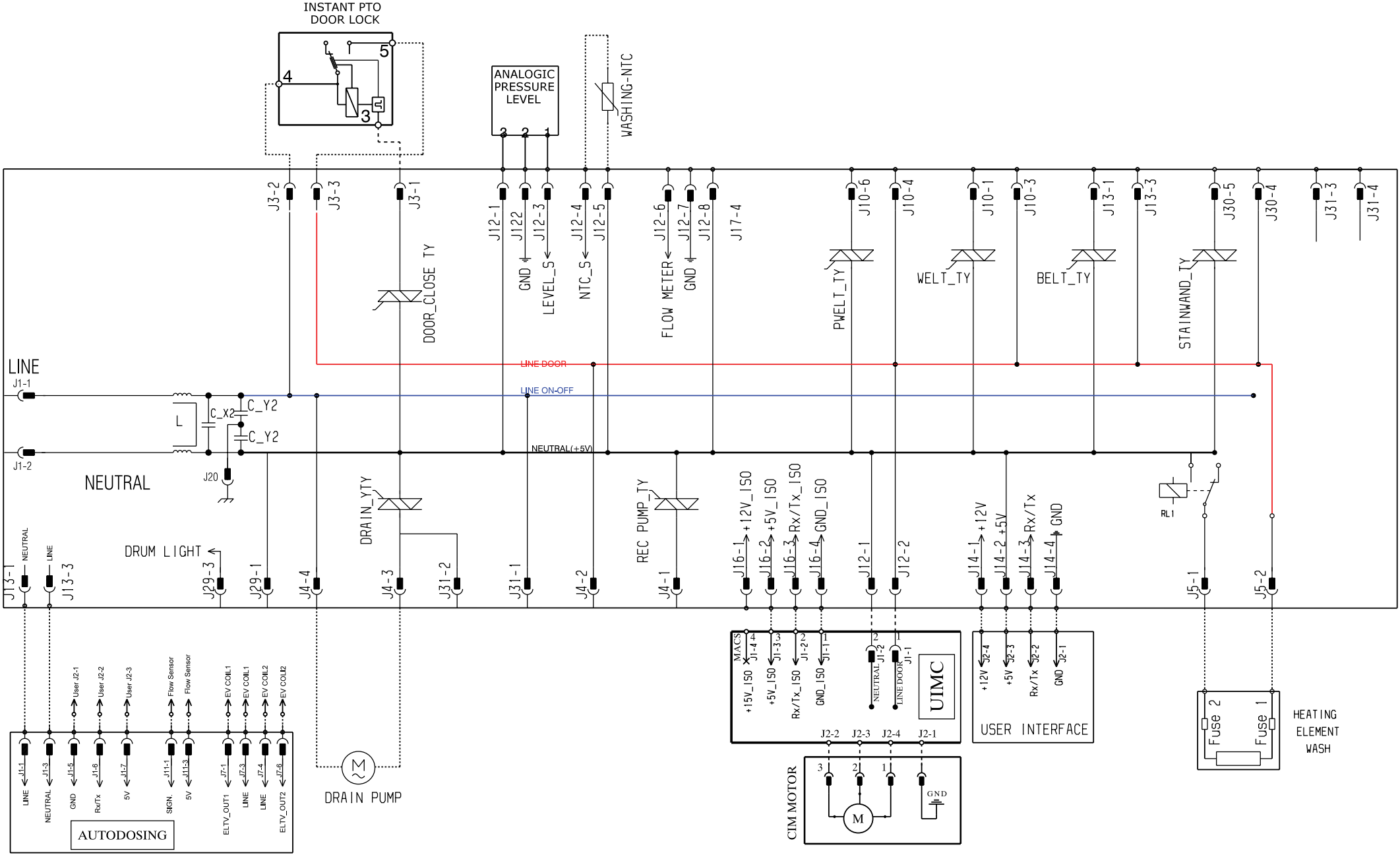
ELECTRIC DIAGRAM EWX14
