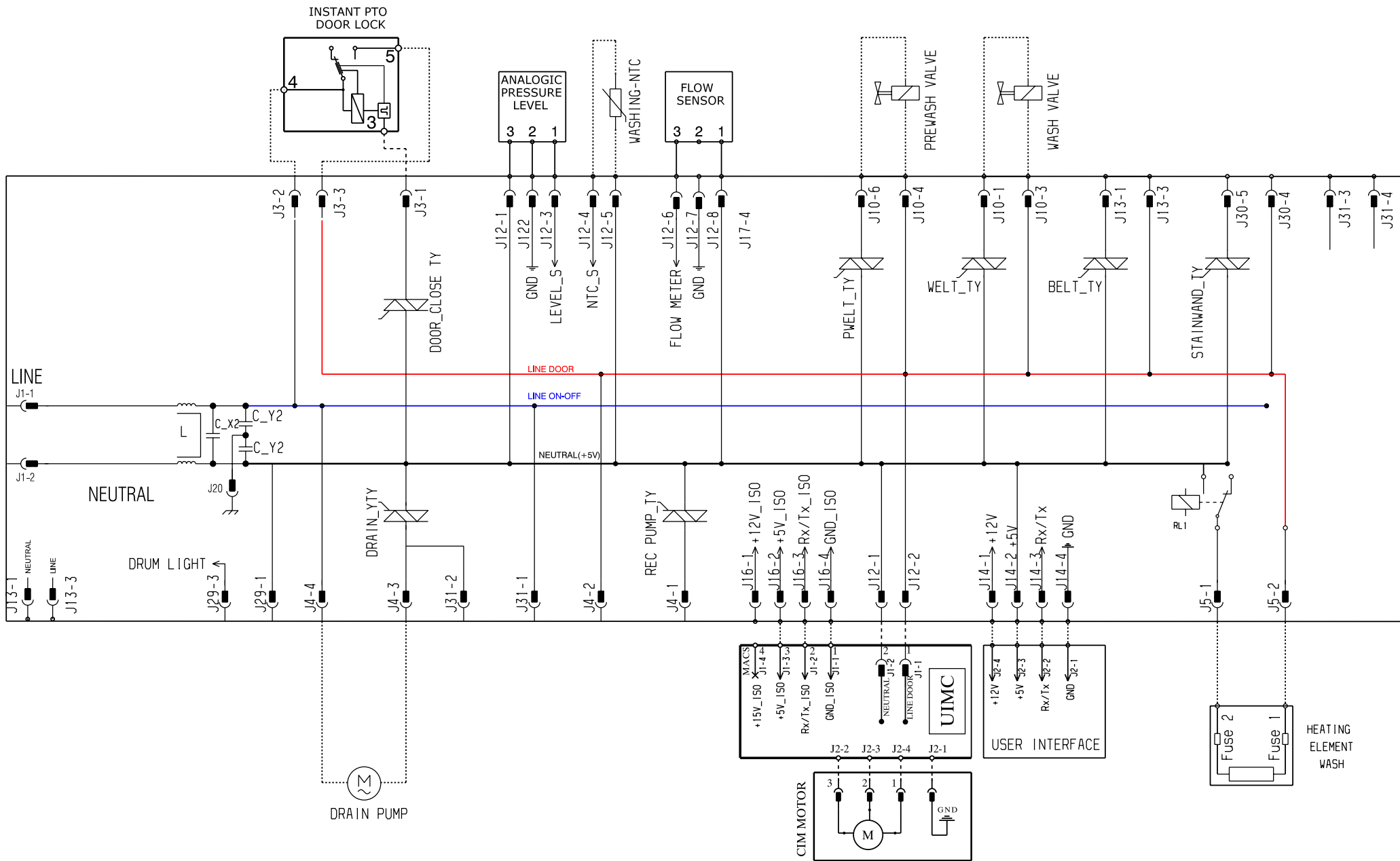
ELECTRIC DIAGRAM EWX14
