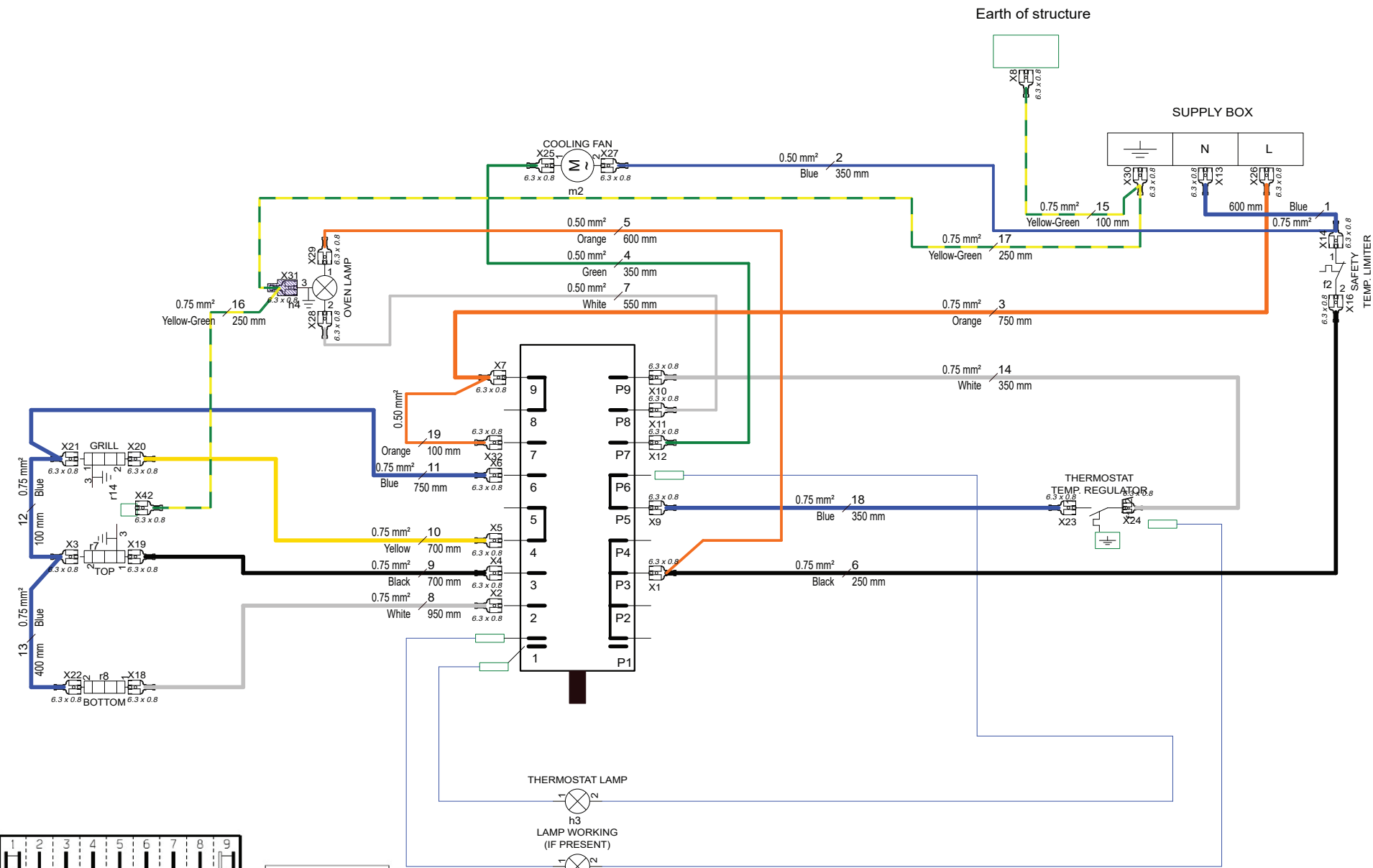
SWITCHING DIAGRAM
