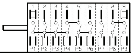
SWITCHING DIAGRAM
