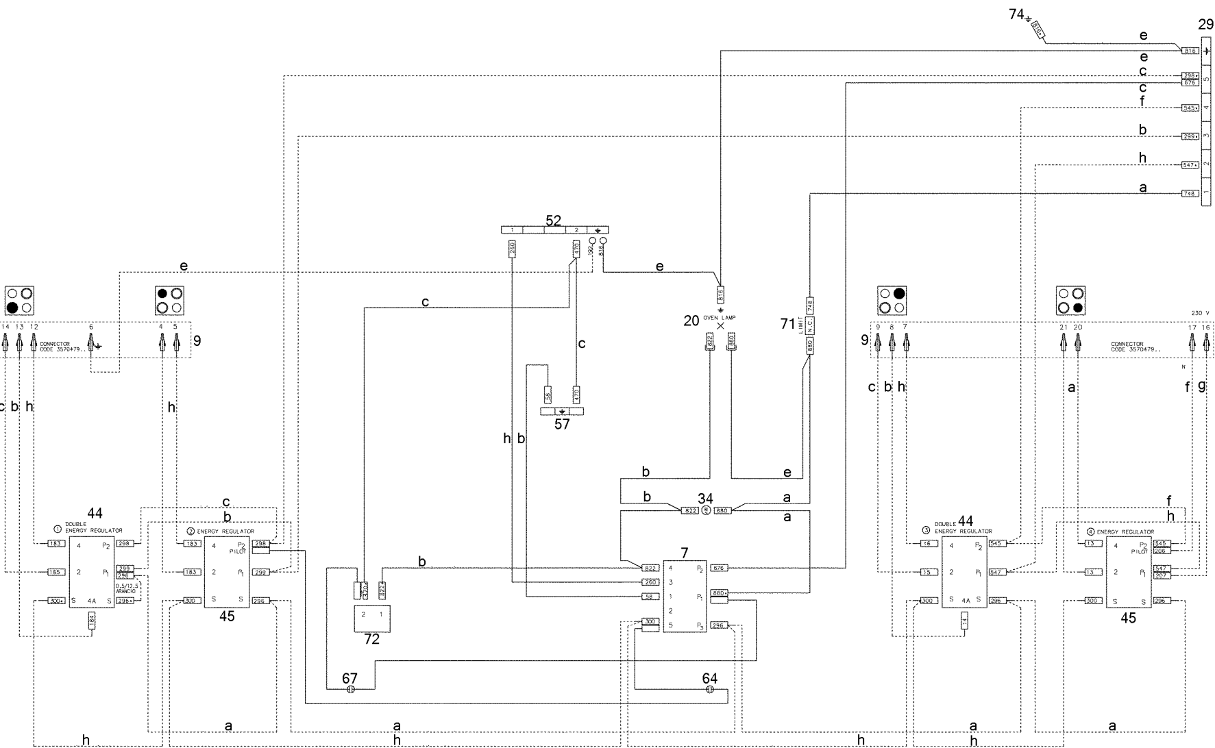
OVEN SWITCH
