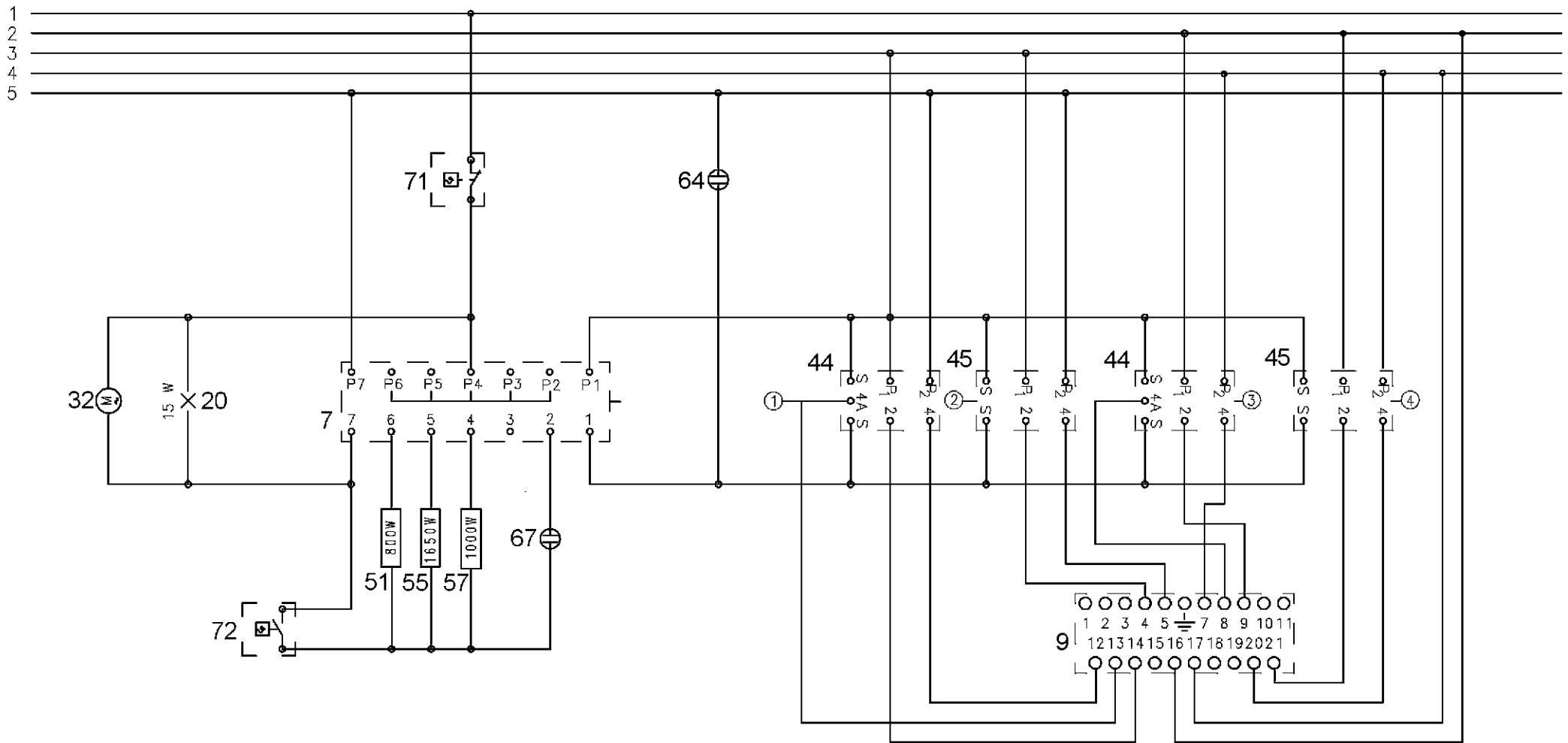
SINGLE ENERGY REGULATOR [2] [4]
