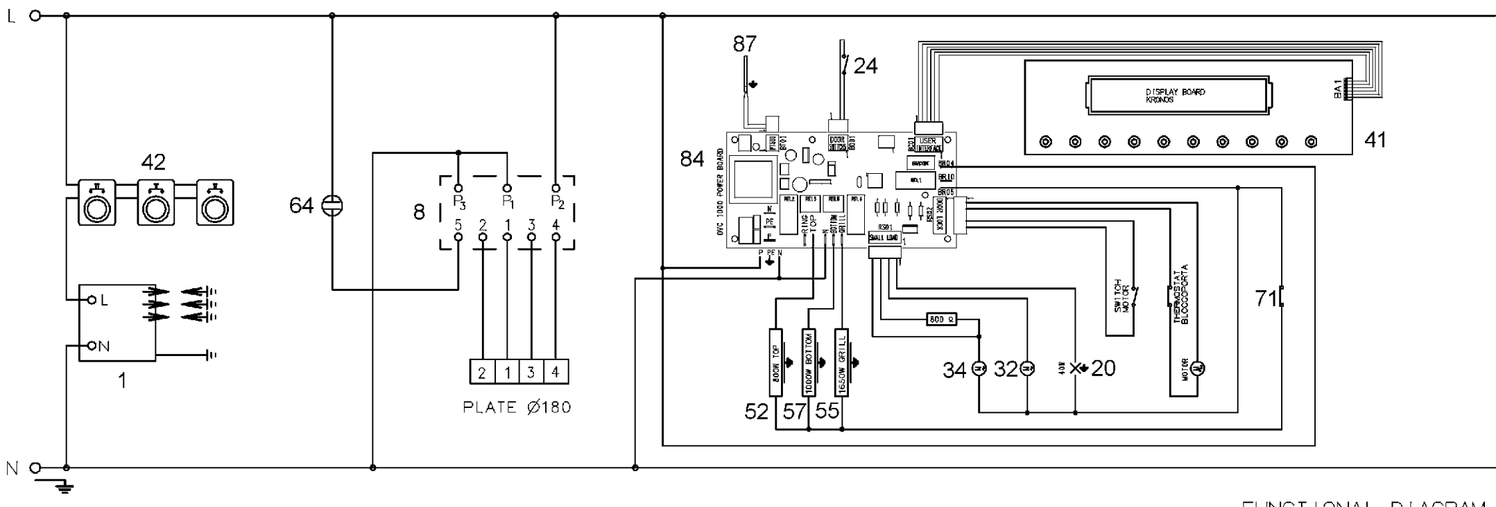
FUNCTIONAL DIAGRAM
