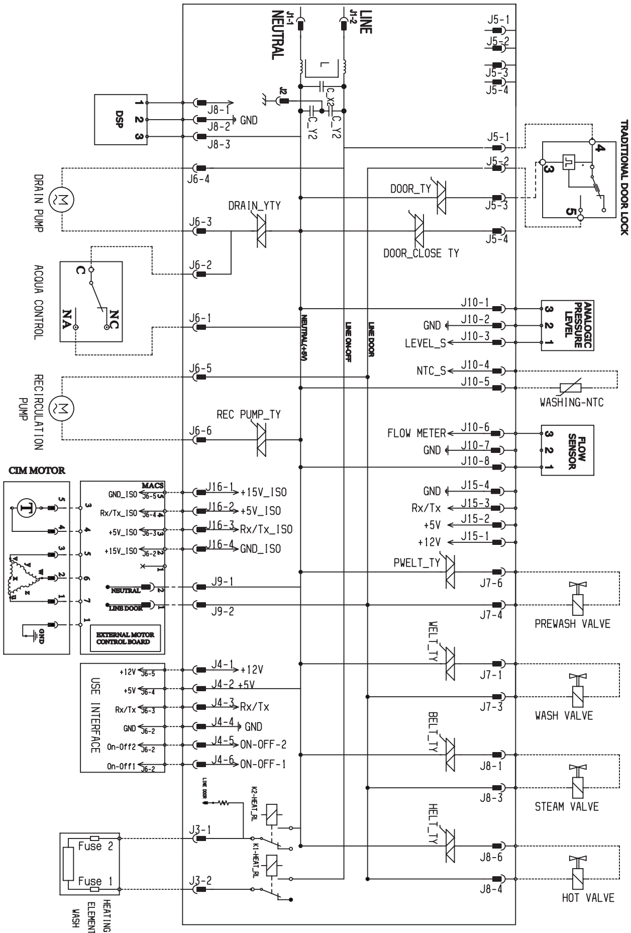
ELECTRIC DIAGRAM EWM10
