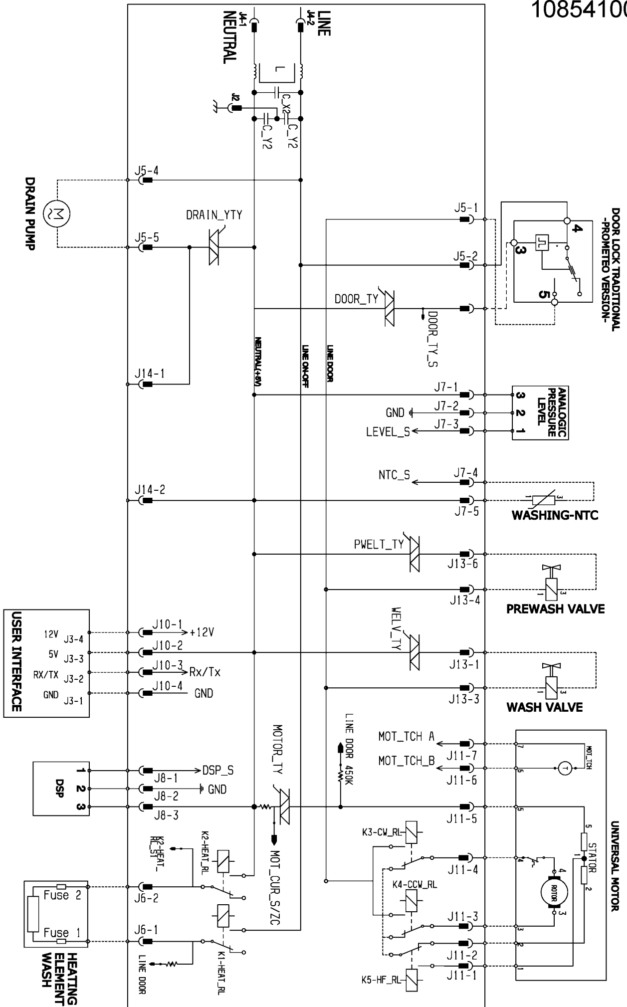
ELECTRIC DIAGRAM -EWM 09-
