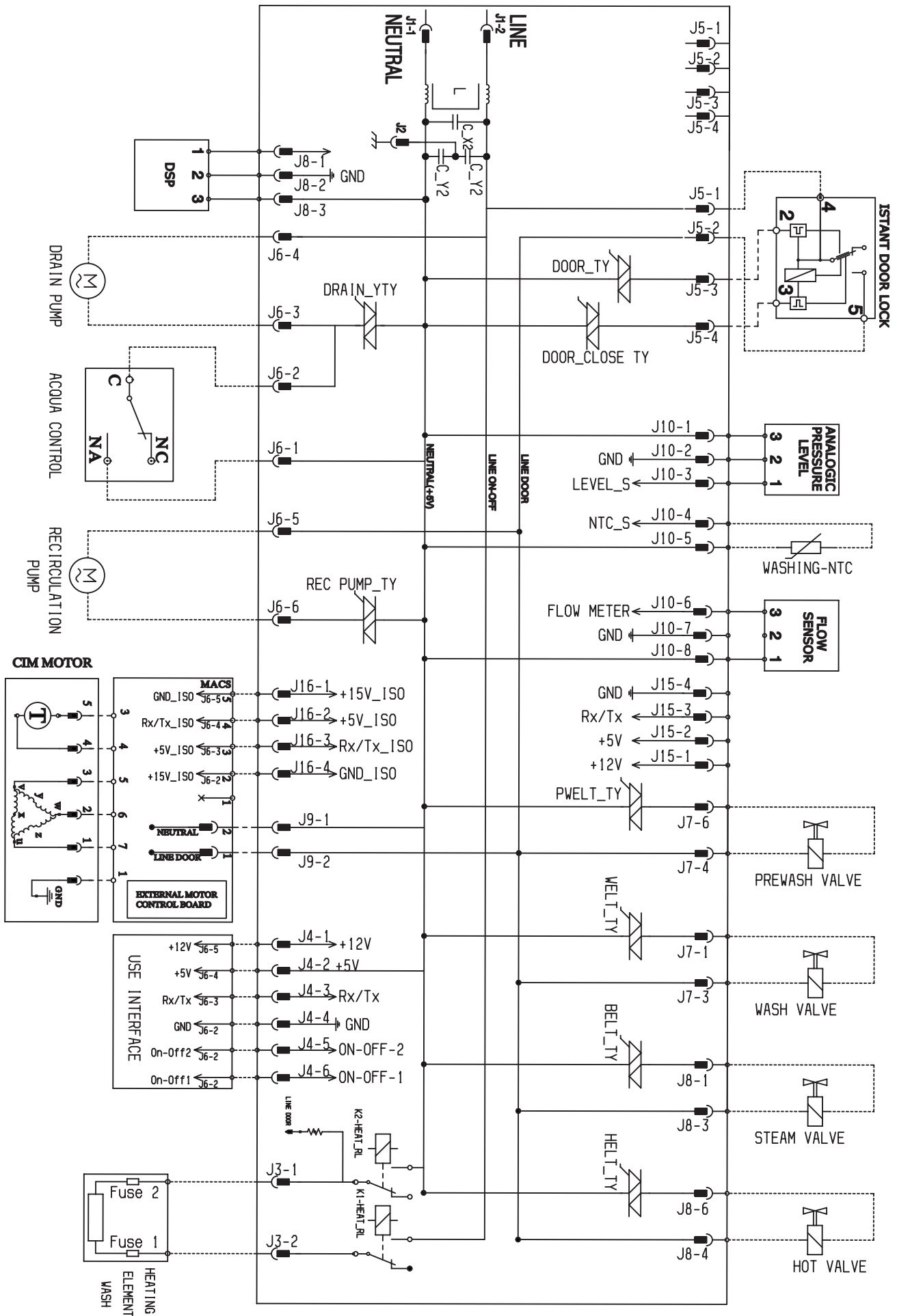
ELECTRIC DIAGRAM EWM10
