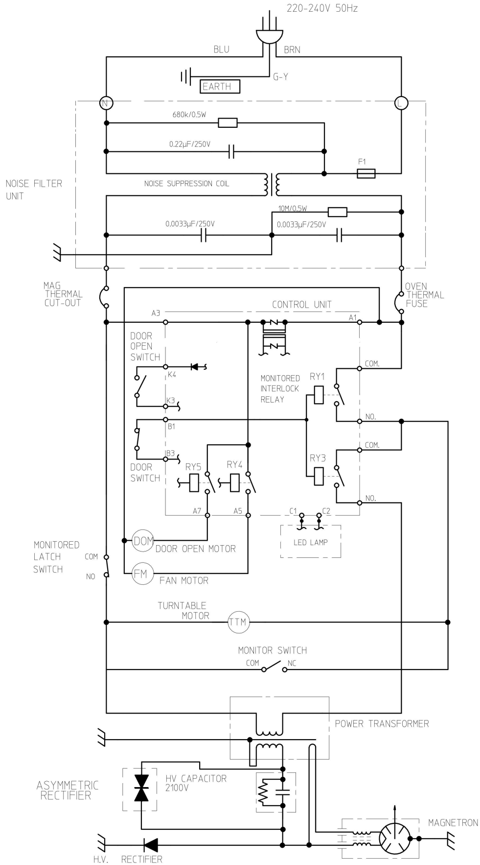
Figure 1 Oven Schematic - OFF Condition, Door Closed
