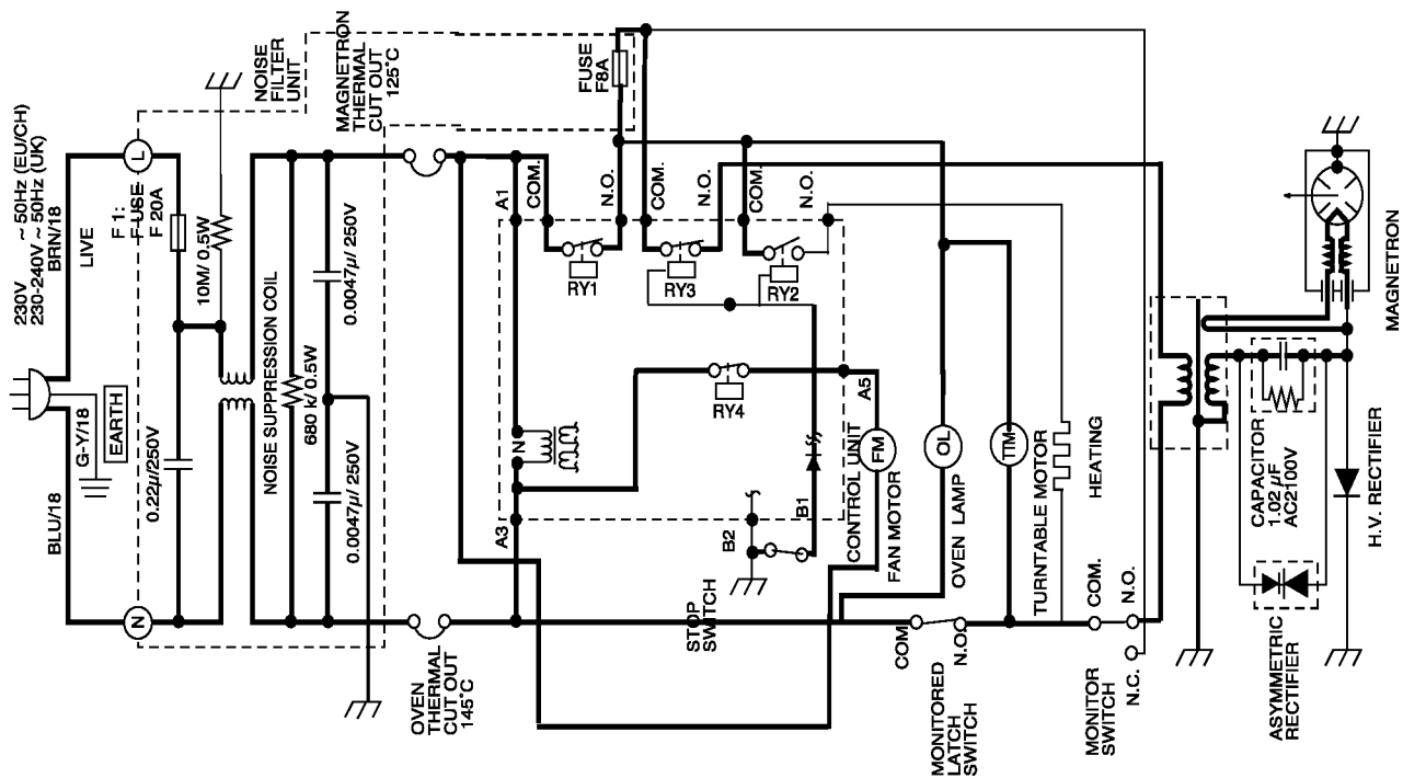
Oven Schematic-ON Condition, Door Closed (Microwave Cooking)
