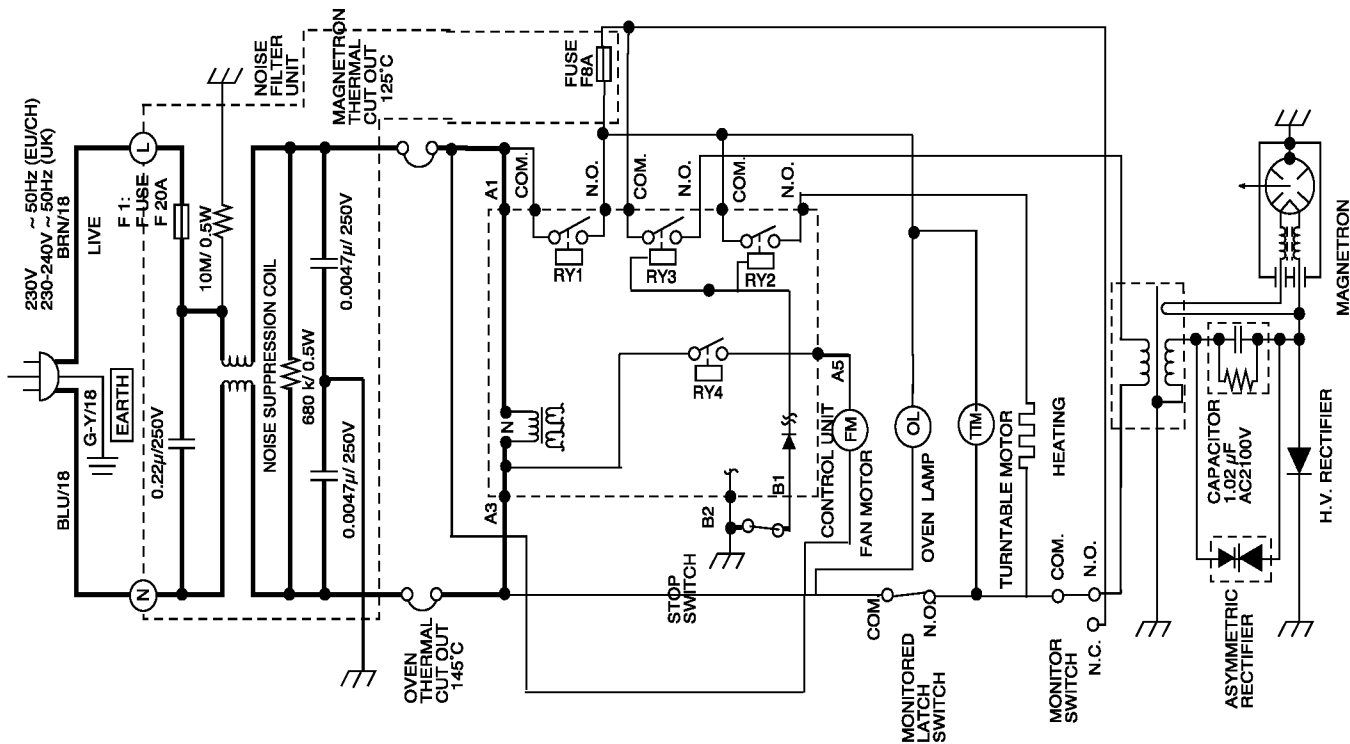
Oven Schematic-OFF Condition, Door Closed
