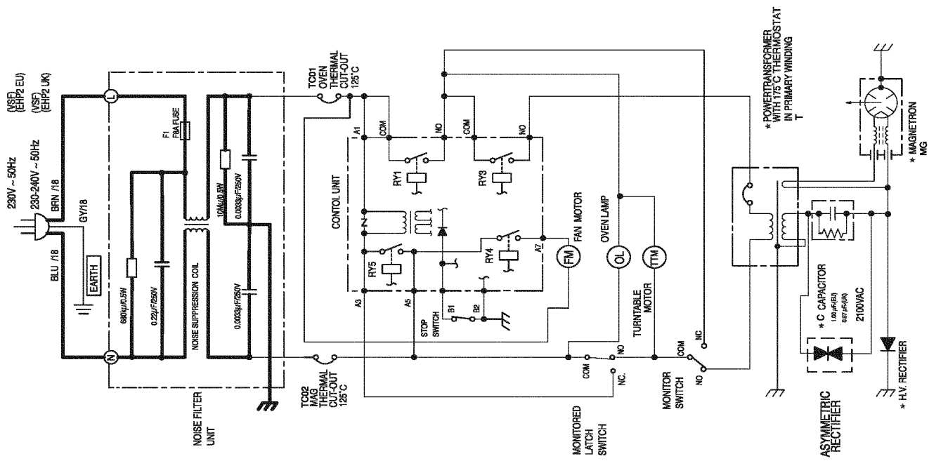
Oven Schematic-OFF Condition, Door Closed.
