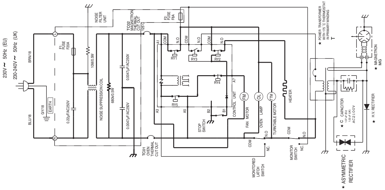
Figure 0-3 Oven Schematic-ON Condition, Door Closed (Grill cooking)
