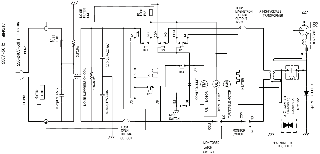
Figure 0-2 Oven Schematic-ON Dual Cooking Condition, (Microwave and Grill mode).
