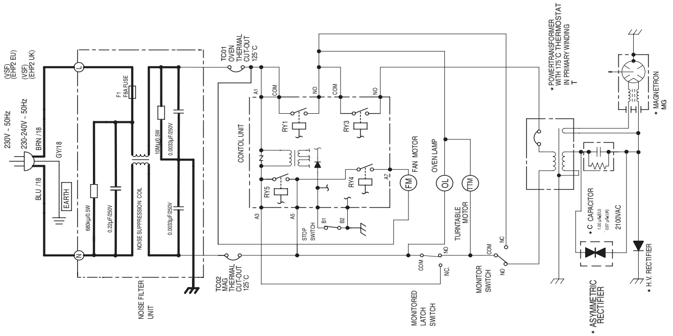
Figure 0-1 Oven Schematic-OFF Condition, Door Closed.
