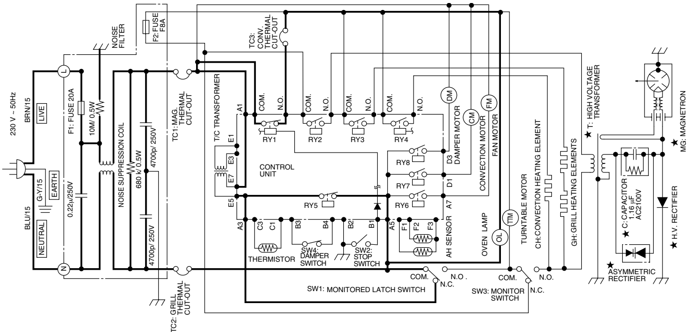
Oven Schematic-Off Condition when the oven door is opened.
