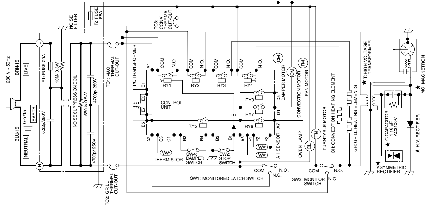
Oven Schematic-Off Condition right after the oven is plugged in.
