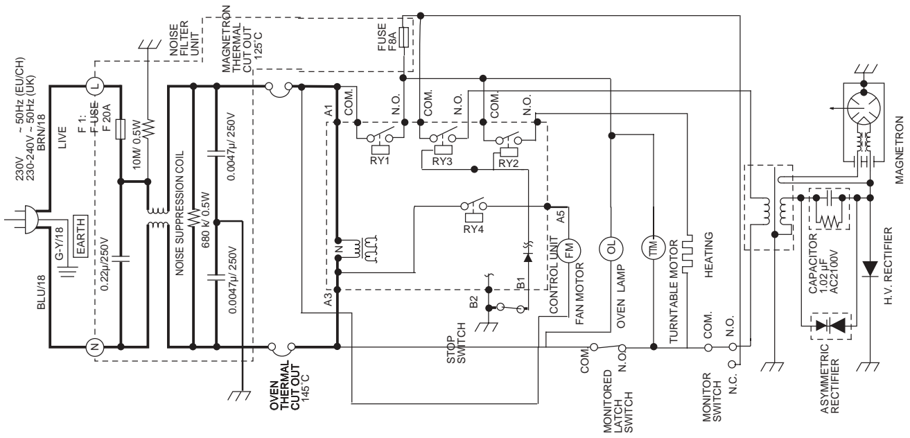
Oven Schematic-OFF Condition, Door Closed
