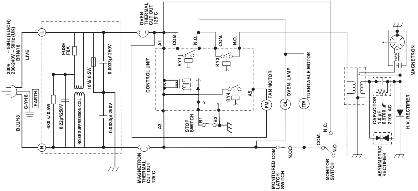
Oven Schematic-OFF Condition, Door Closed.
