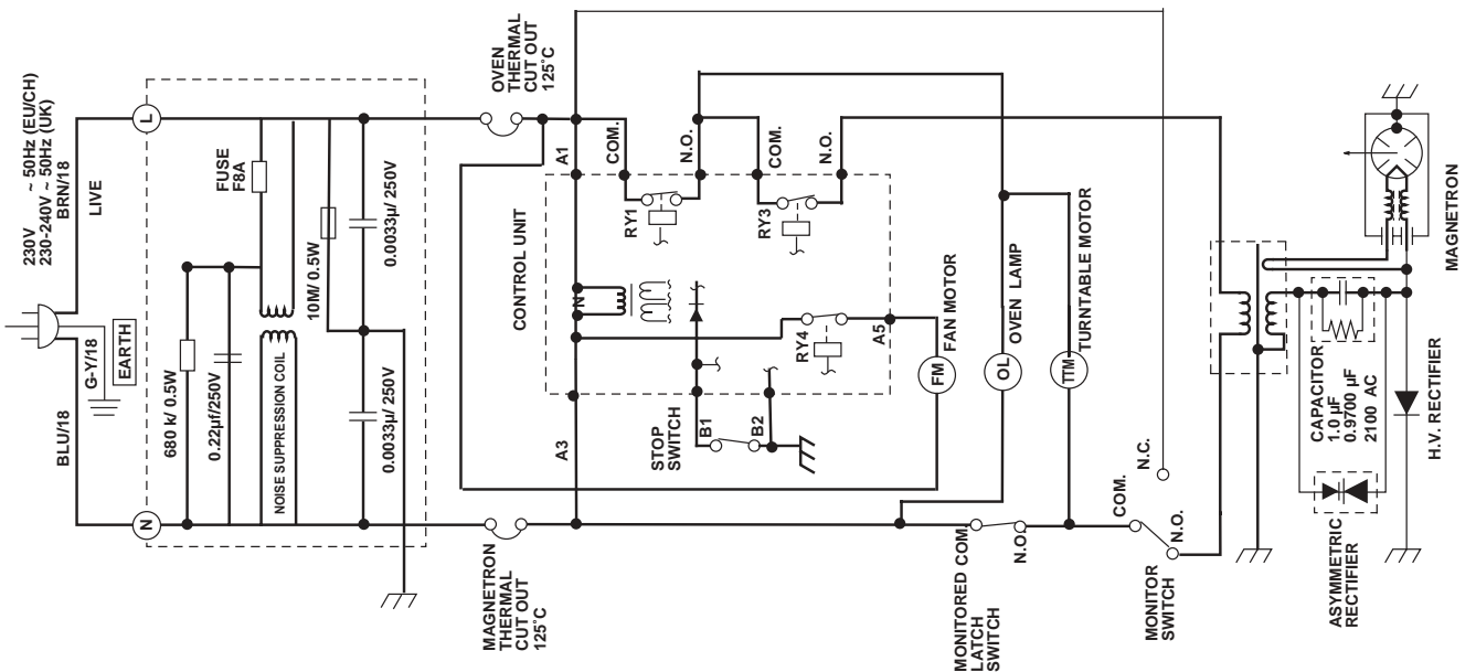
Oven Schematic-ON Condition, Door Closed.
